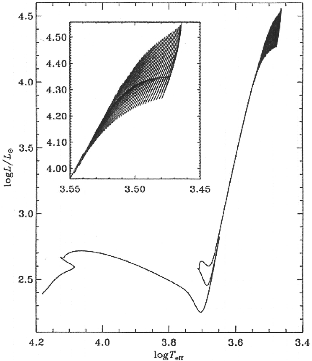
Evolutionary track for a 4 M_{\odot} star from the ZAMS to the AGB stage. The insert show the late, thermally pulsating AGB phase.
